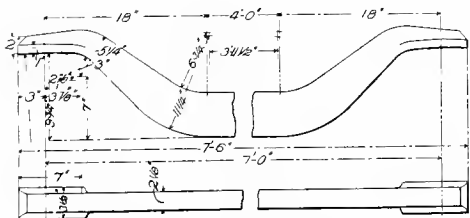
Figs. 4889-90. EQUALIZING-BAR.
